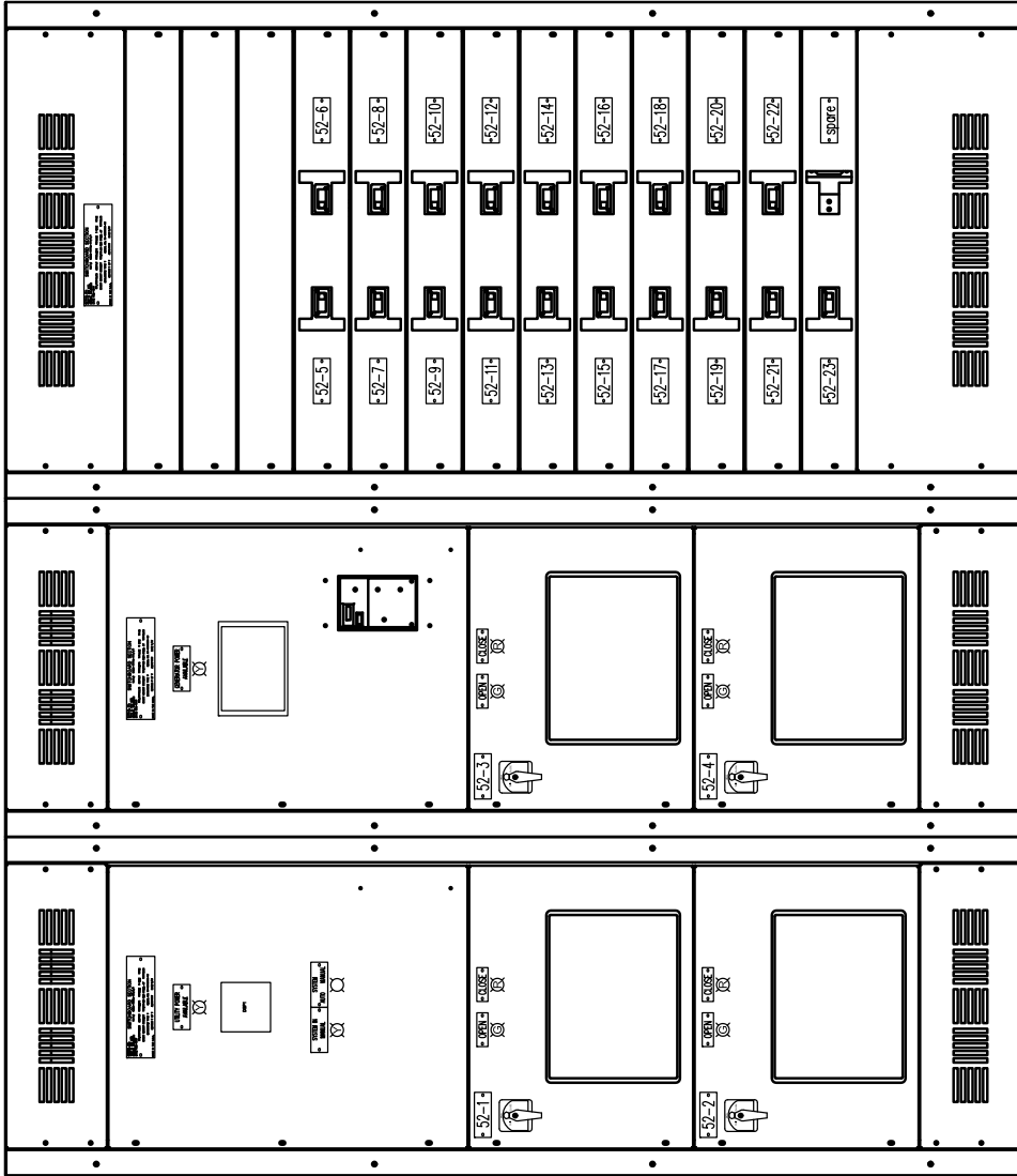
SECTION -101
